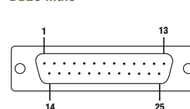
DB25 male
