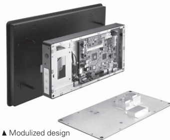
▲ Modulized design
