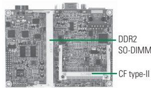
▲ Rear view
