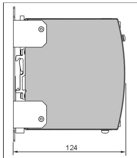
Fig. 23-6 Wall/panel mounting, side view
