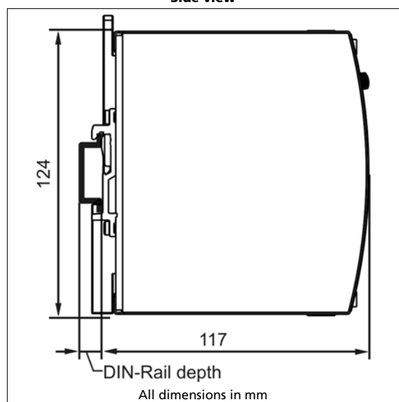
Fig. 22-2 Side view
