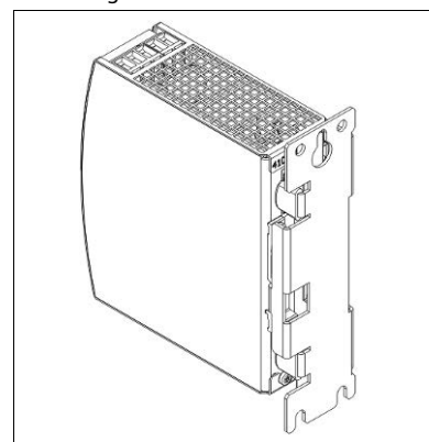
Fig. 23-3 Isometric view
